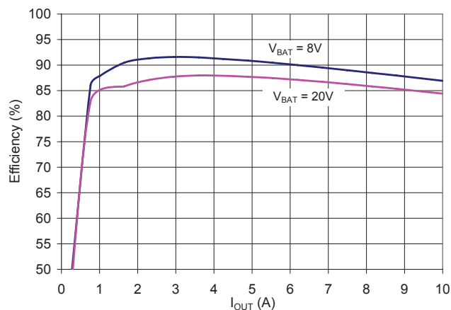
1.2V Efficiency (Continuous Conduction Mode) (High Efficiency Design, Page 21)
