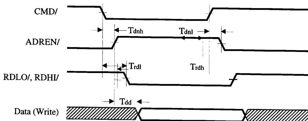
82C451 AD Bus Multiplexer Timing
