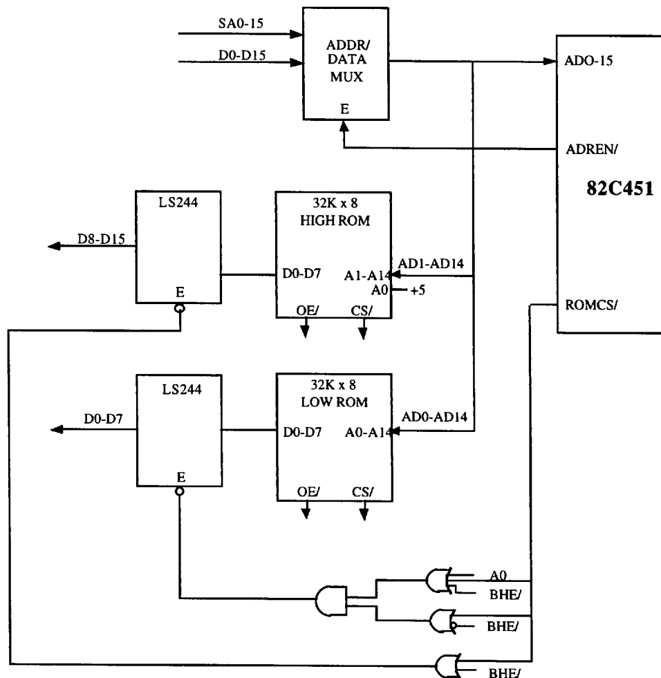
Block Diagram - 16 bit BIOS ROM (32k x 8 ROMs)
