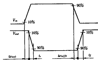
WAVEFORMS
