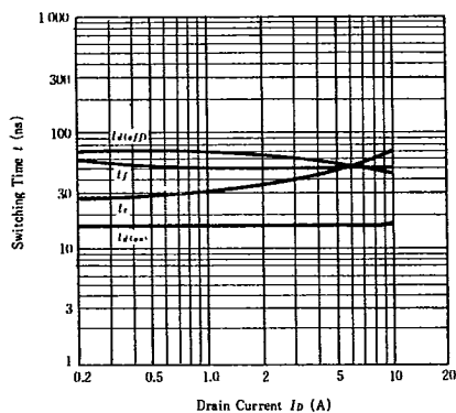
SWITCHING CHARACTERISTICS
